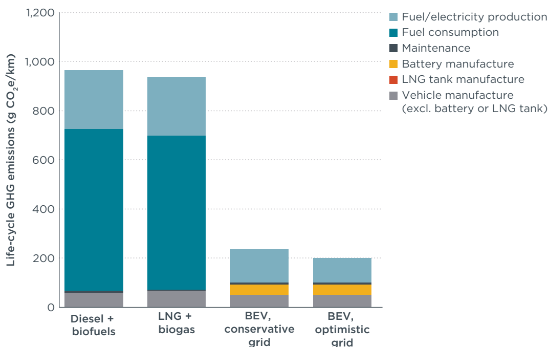
2030 40-tonne tractor-trailer – diesel and LNG versions compared to BE version using (a) a conservative grid scenario, or (b) an optimistic (greener) electricity grid
